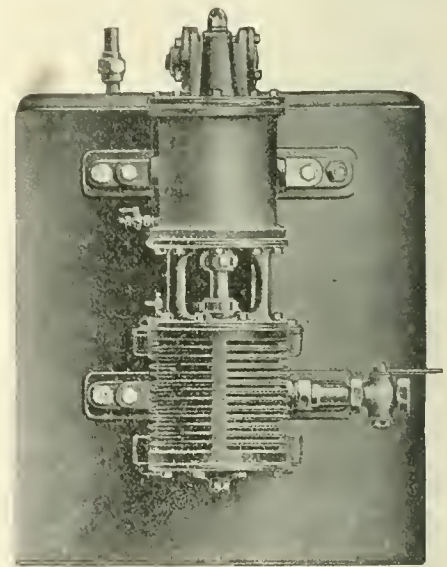
A NEAT ARRANGEMENT OF AN AIR PUMP MOUNTED ON A MAIN RESERVOIR IN AN AIR BRAKE REPAIR ROOM.
